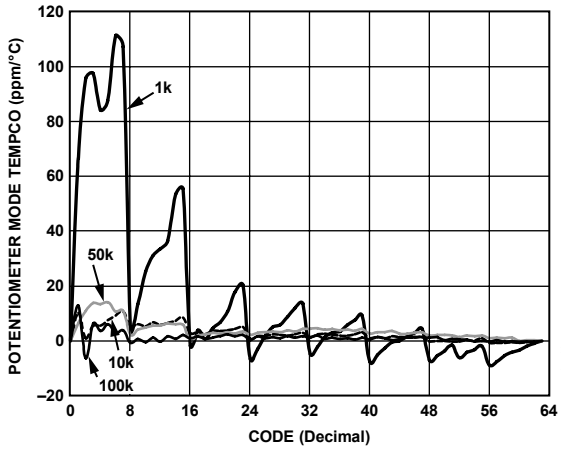
Figure 18. Potentiometer Mode Tempco ( \Delta V_W \times 10^5 )/( V_W \times \Delta T ) vs. Code
