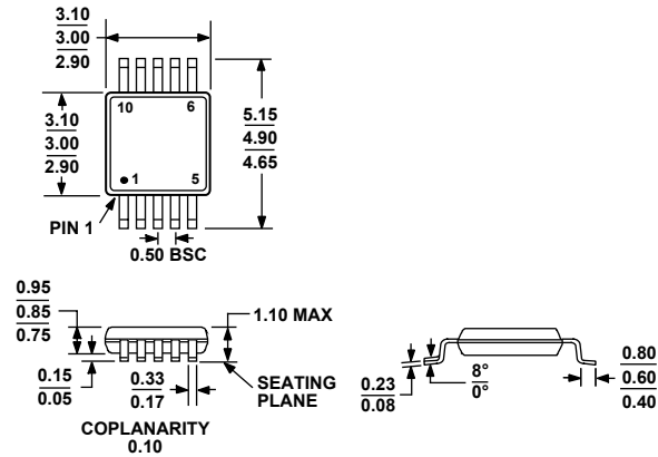
Figure 46. 10-Lead Mini Small Outline Package [MSOP] (RM-10)
